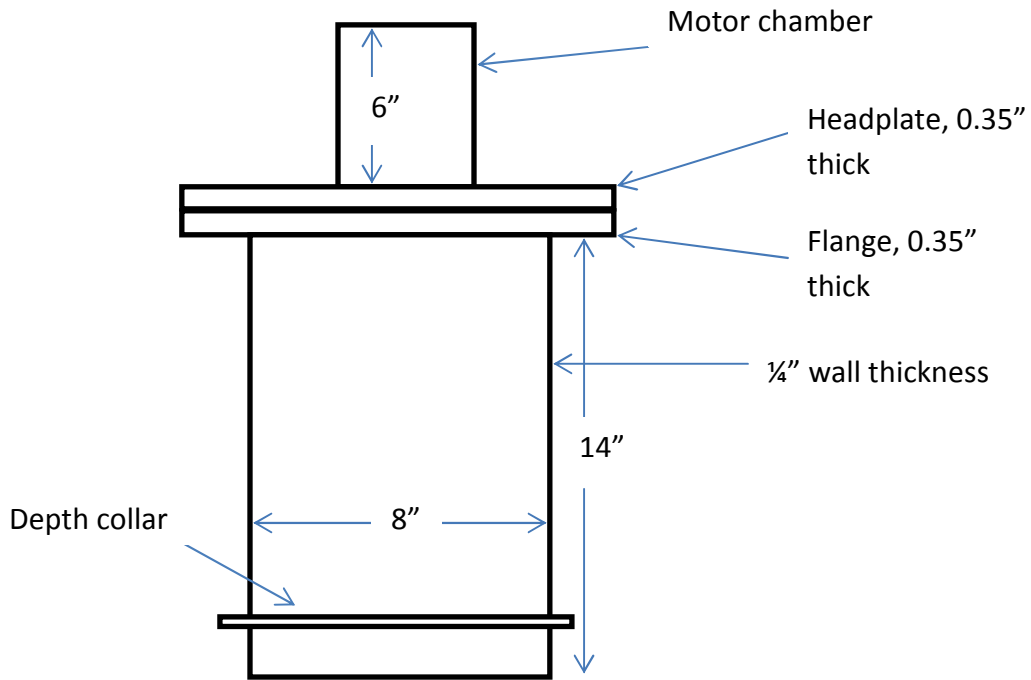
Benthic Chamber Dimensions
