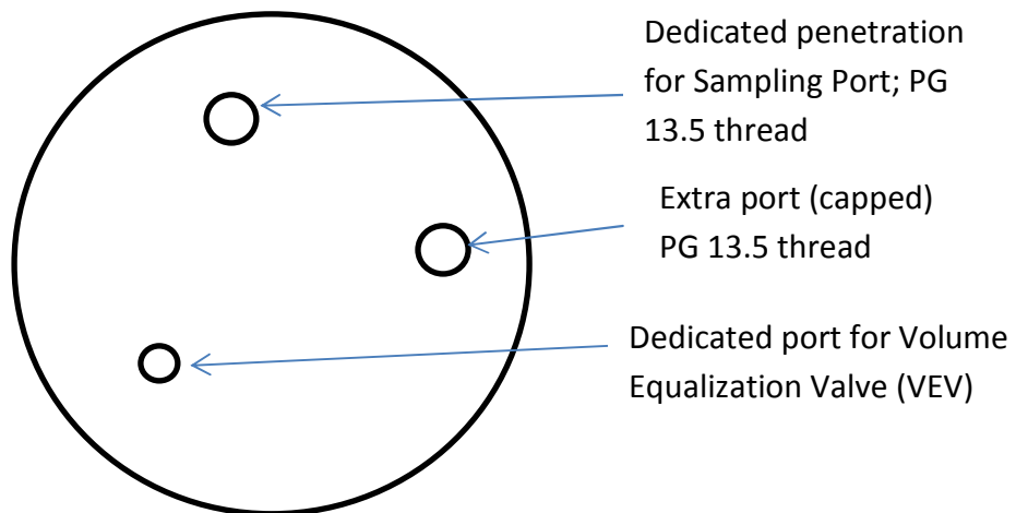
Headplate Penetrations
